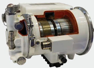
AC GENERATOR
